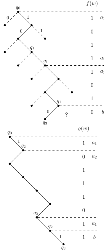
FIG. 6.3. The trees generated by w = a_1a_2a_1b
